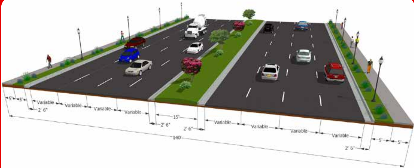
8- or 10-Lane, divided roadway with a planted median, curbs, gutters, planted strips, pedestrian level lighting and sidewalks on both sides
